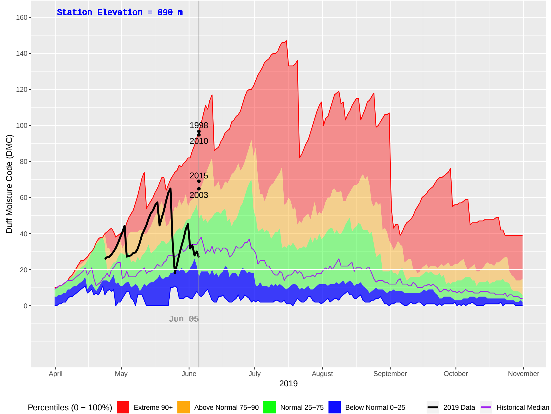
ISKUT (112) : Historical (1979–2018), Current (2019) Daily Duff Moisture Code (DMC)
