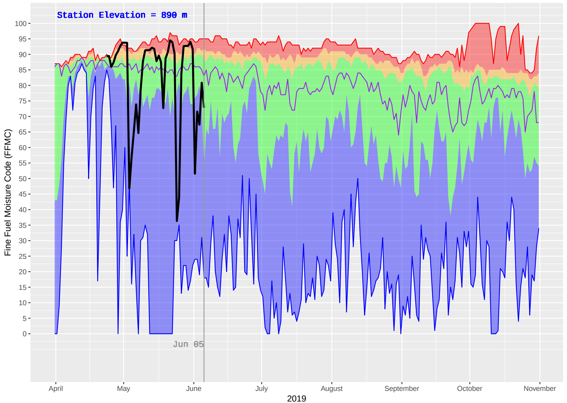
ISKUT (112) : Historical (1979–2018) and Current (2019) Daily Fine Fuel Moisture Code (FFMC)
