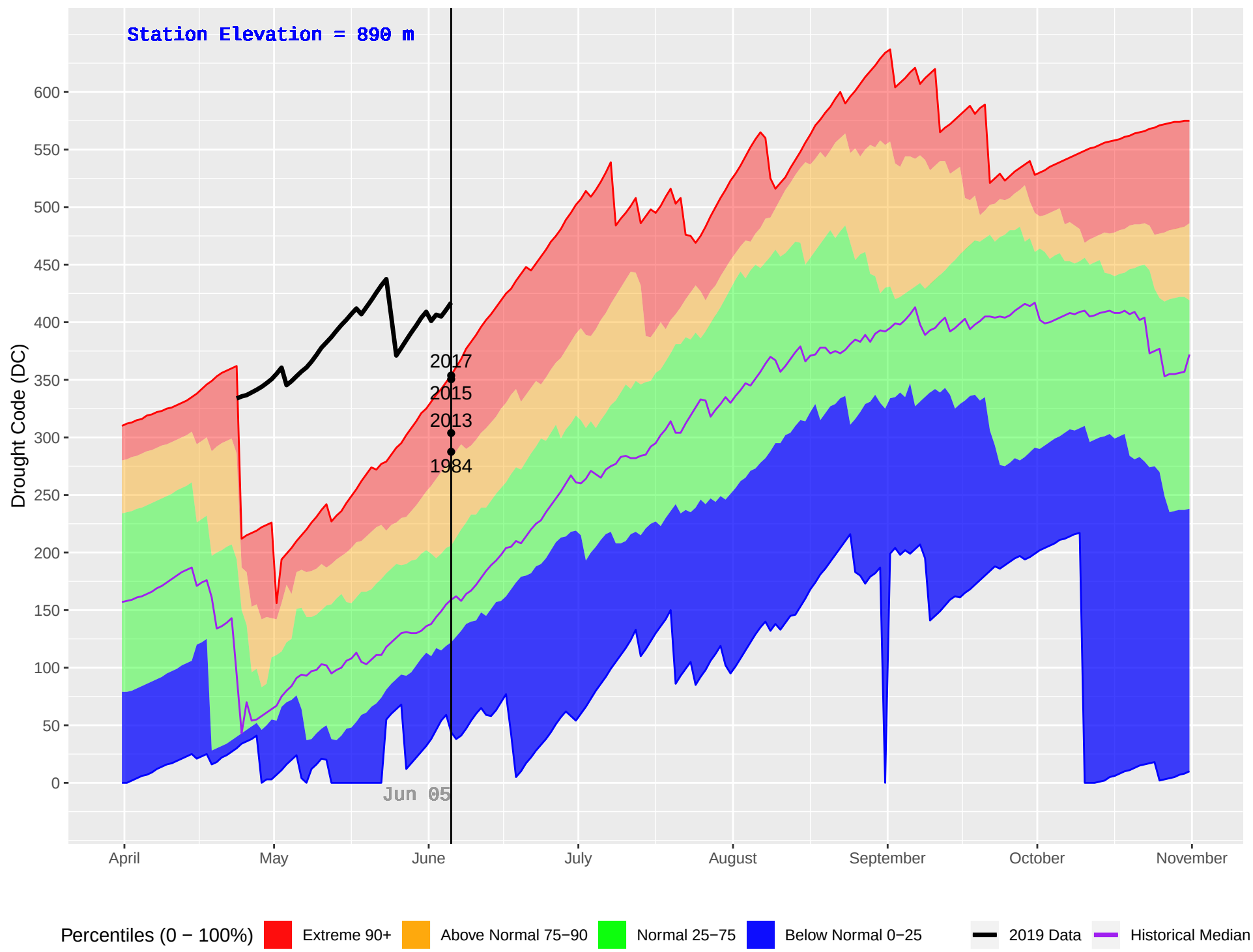
ISKUT (112) : Historical (1979–2018) and Current (2019) Daily Drought Code (DC)
