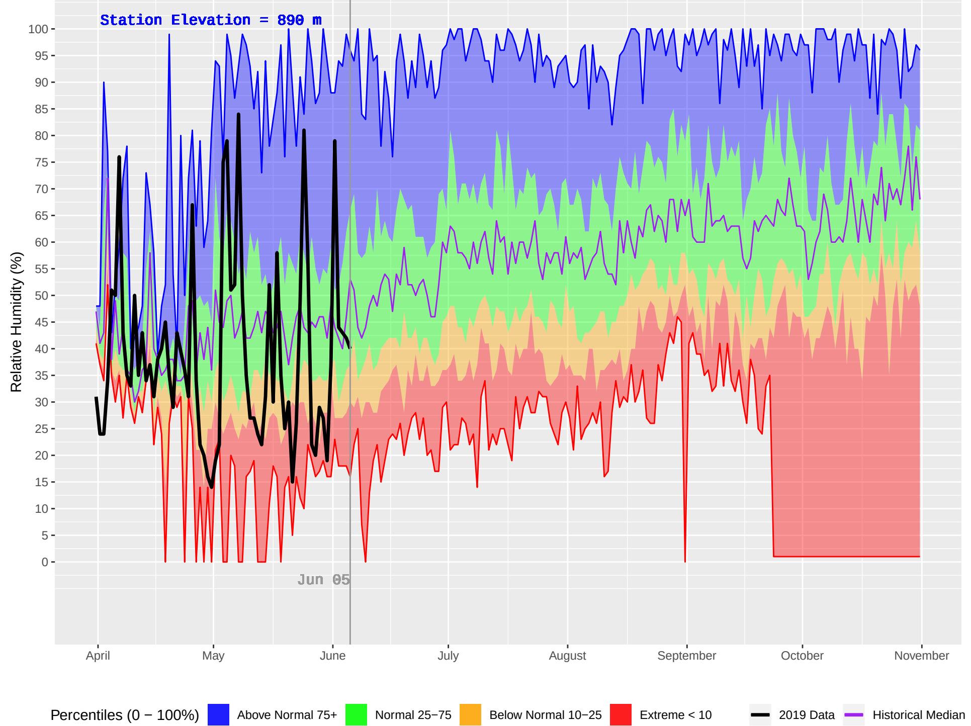
ISKUT (112) : Historical (1979–2018) and Current (2019) Daily Relative Humidity
