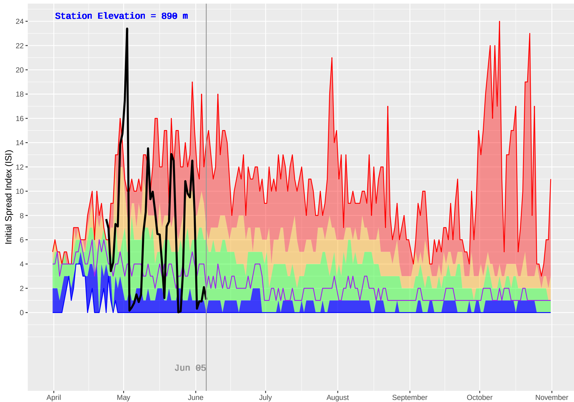
ISKUT (112) : Historical (1979–2018) and Current (2019) Daily Initial Spread Index (ISI)
