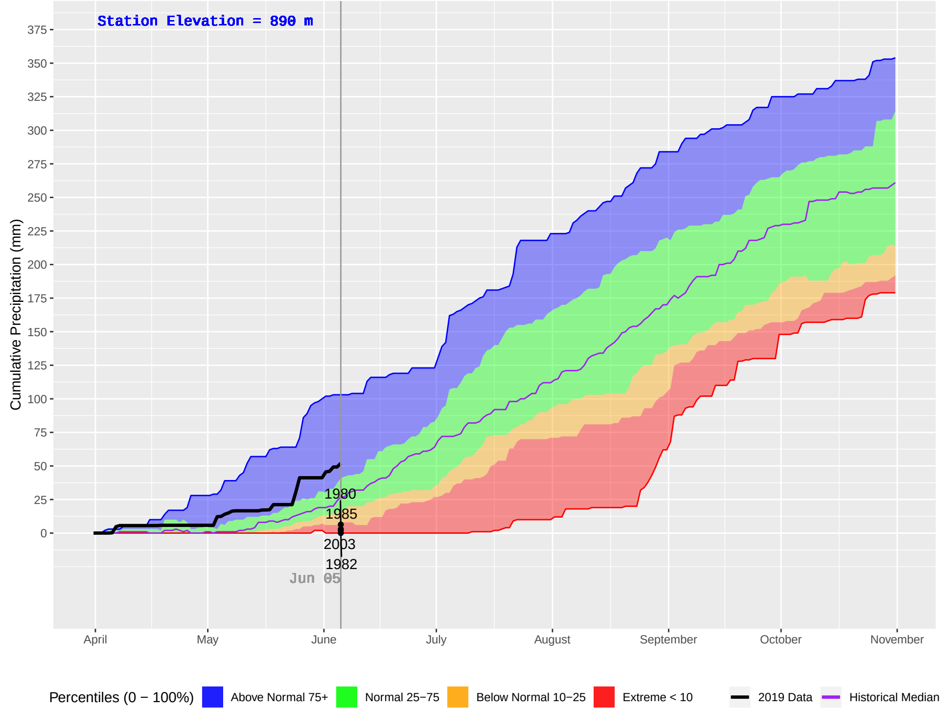
ISKUT (112) : Historical (1979–2018), Current (2019) Daily Cumulative Precipitation
