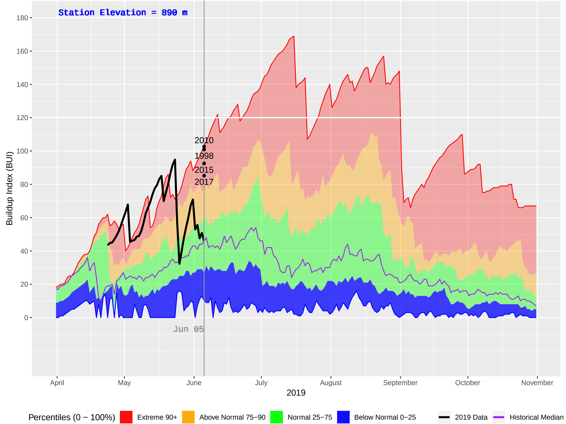
ISKUT (112) : Historical (1979–2018), Current (2019) Daily Buildup Index (BUI)
